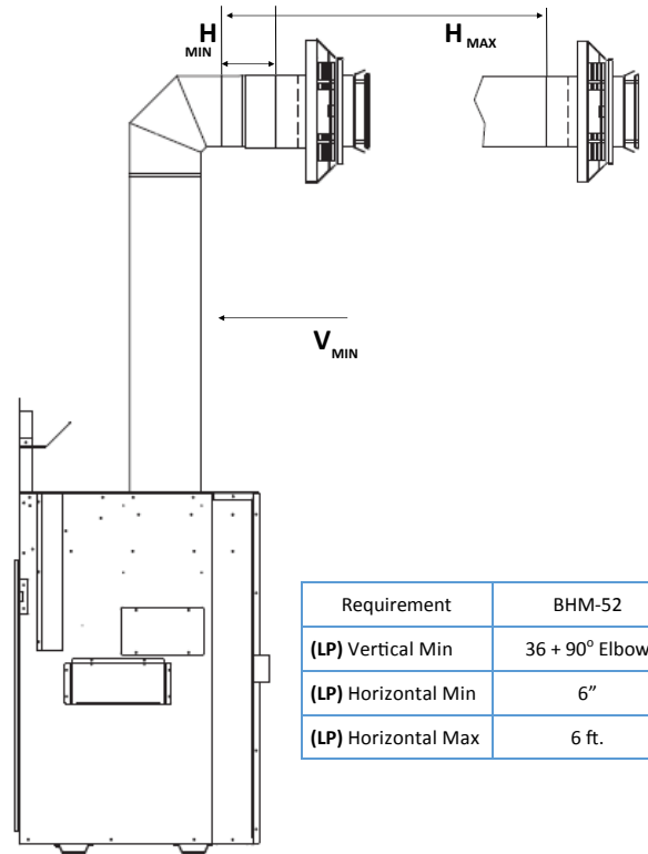
Vertical Terminations with Reducer
